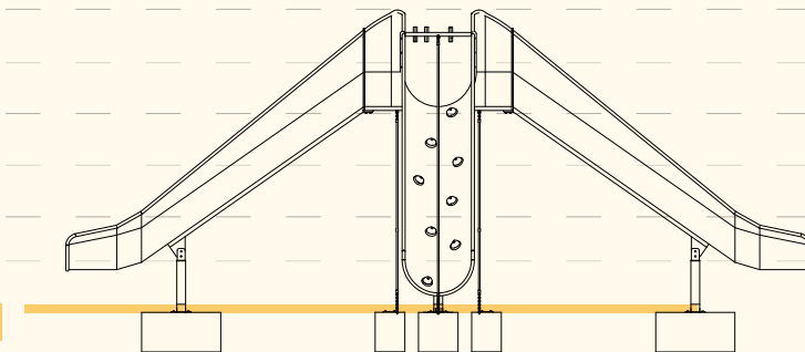
Surface mount Installation -10cm
